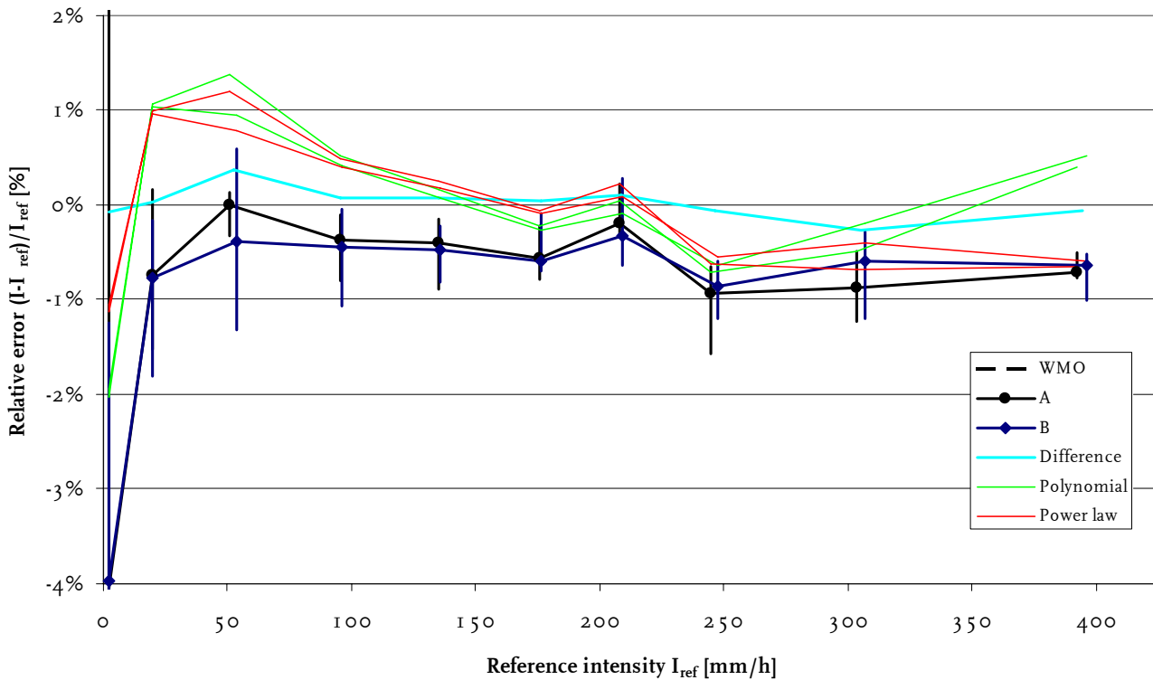
Figure 13: Summary of the test results of the MRW500 instruments showing the averaged test results of both instruments versus the reference intensity, the relative difference between the results obtained for both instruments, and the errors after a correction using the second order polynomial or power law fit has been applied to the data.
