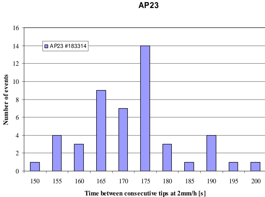
Figure 9: Histogram of the observed time intervals between consecutive tips for the AP23 instrument at 2 mm/h. The time denoted at the x-axis is the end time of the time interval; hence the entry at 150 denotes the tip that occurred 150 s after the previous tip. Note that in this case the tip at 200 occurred after 205 s since all tips outside the range are placed in the limiting bins.
