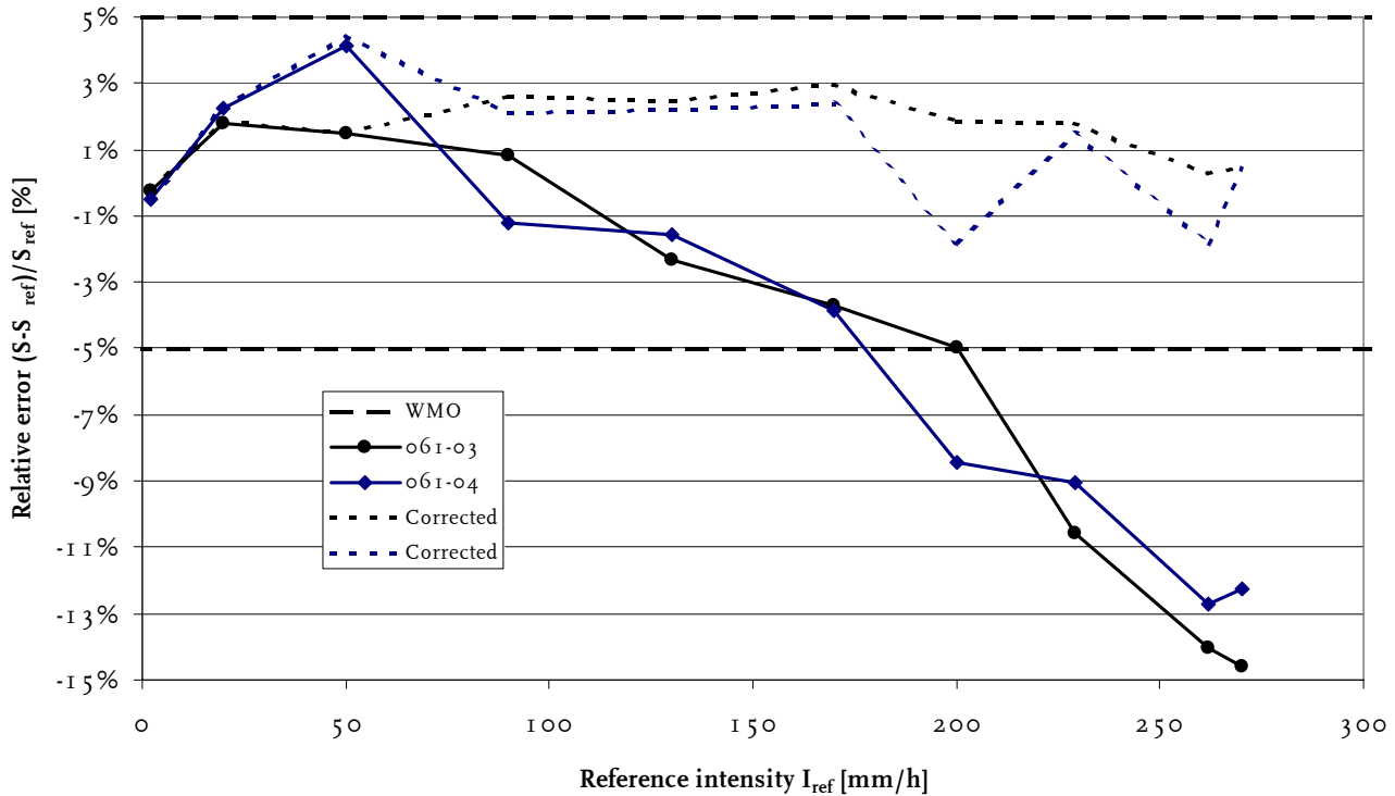
Figure 58: Summary of the test results of the Neerslagmeter instruments showing the relative difference of the total precipitation sums of the averaged test results of both instruments versus the reference. Solid lines show the raw sensor results, whereas in the dashed lines emptying is filtered out.
