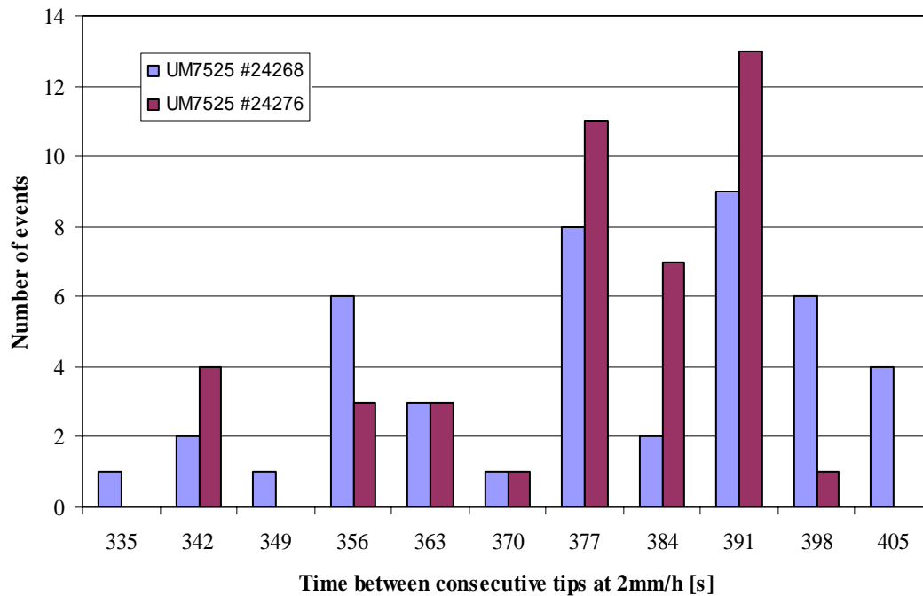
Figure 33: Histogram of the observed time intervals between consecutive tips for both UM7525 instruments at 2 mm/h. The time denoted at the x-axis is the end time of the time interval, hence 1 tip occurs between 328 and 335 s.
