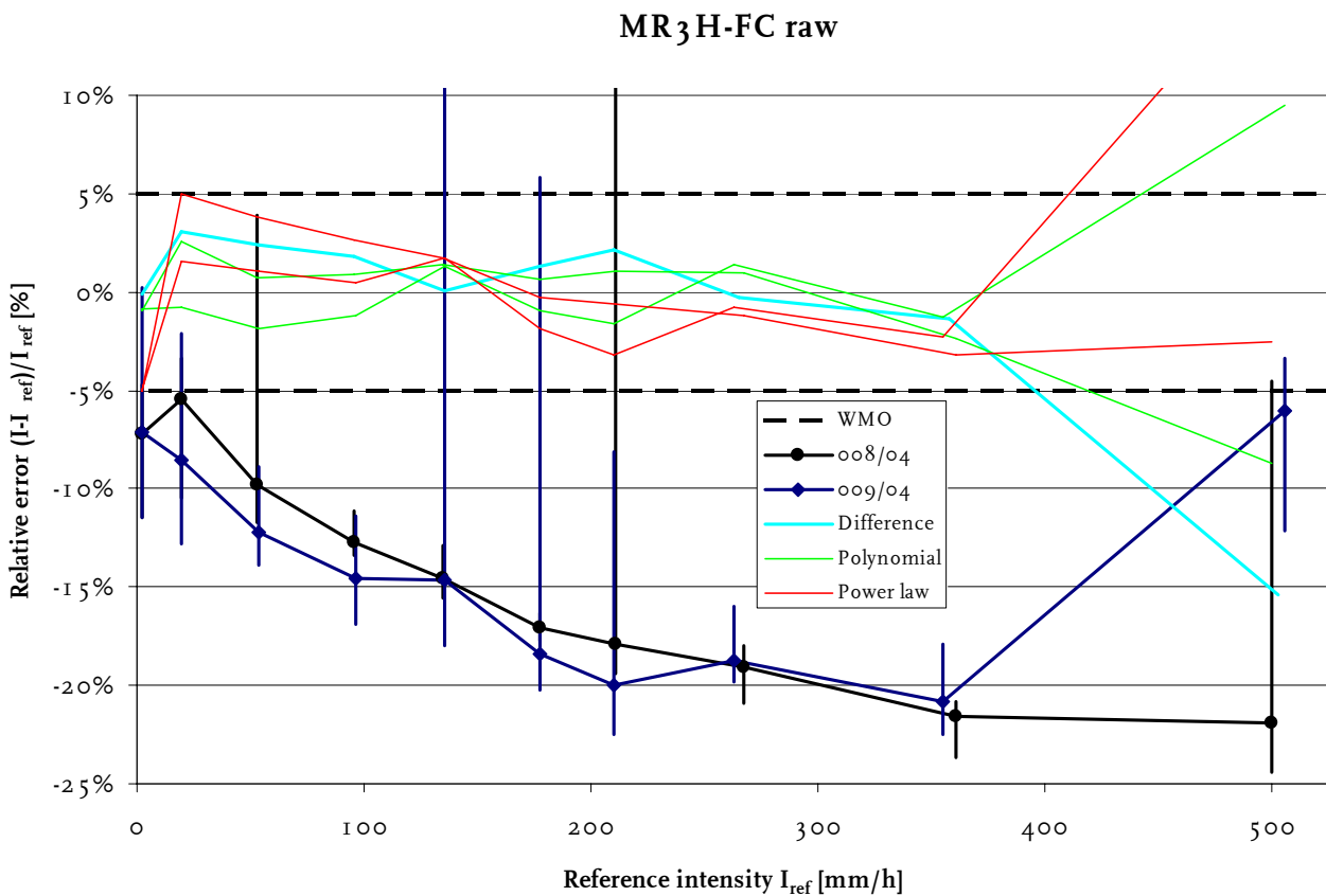
Figure 17: Same as Figure 16, but now for the raw read output of the MR3H-FC instruments.
