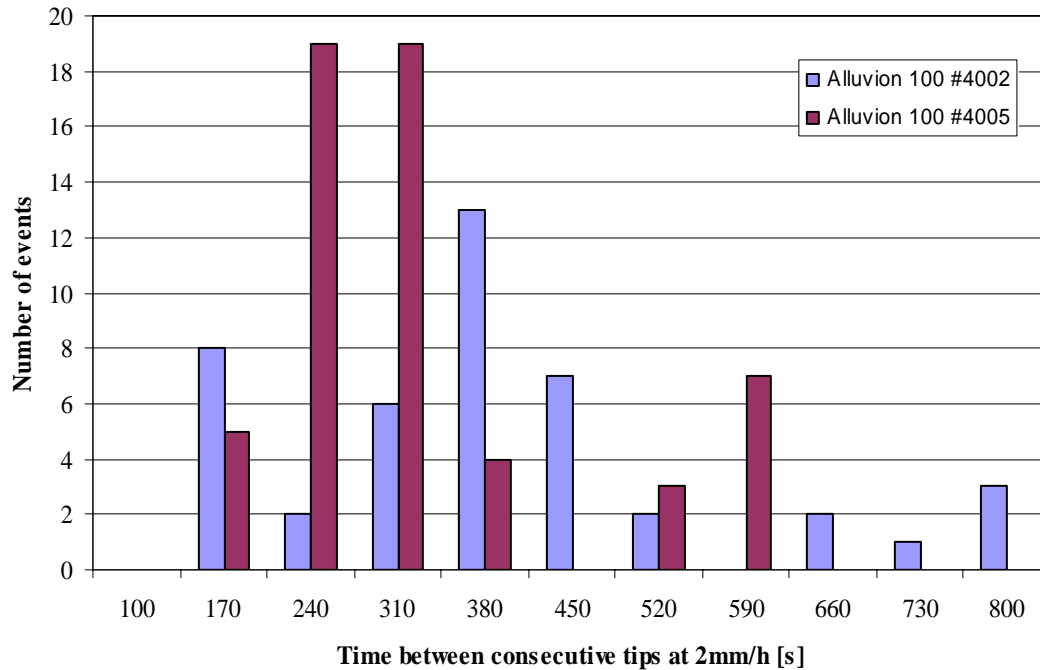
Figure 11: Histogram of the observed time intervals between consecutive increments for both Alluvion 100 instruments at 2 mm/h. The time denoted at the x-axis is the end time of the time interval.
