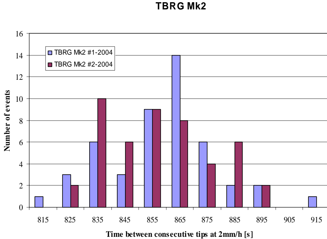
Figure 31: Histogram of the observed time intervals between consecutive tips for both TBRG Mk2 instruments at 2 mm/h. The time denoted at the x-axis is the end time of the time interval, hence 1 tip occurs between 805 and 815 s.
