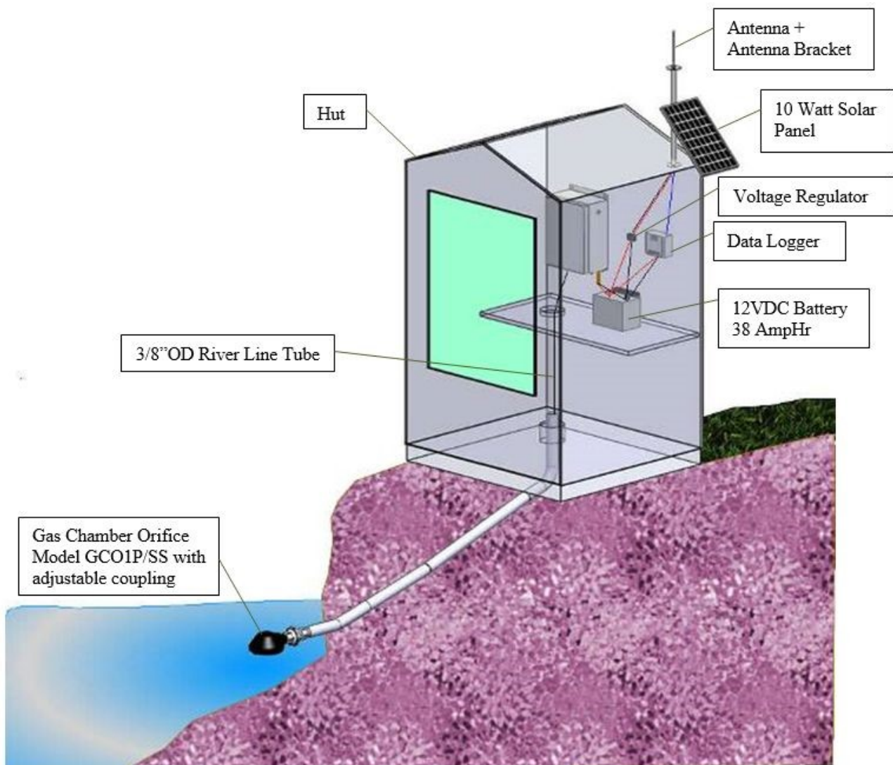
HS40 Compact Typical Installation
