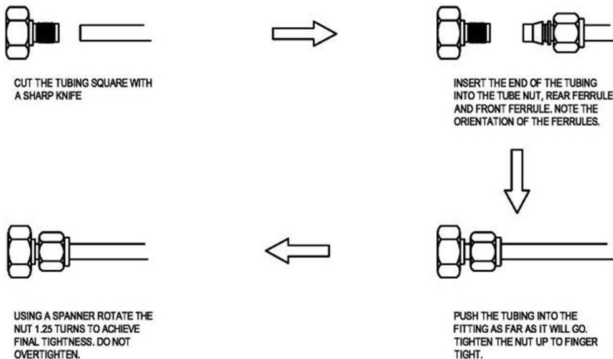
TYPICAL TIGHTENING PROCEDURE FOR RIVERLINE FITTINGS
