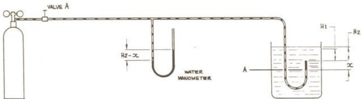
Figure 5 - With gas supply cut off. Head increased from H1 to H2, gas is forced down the tube by an amount X.
