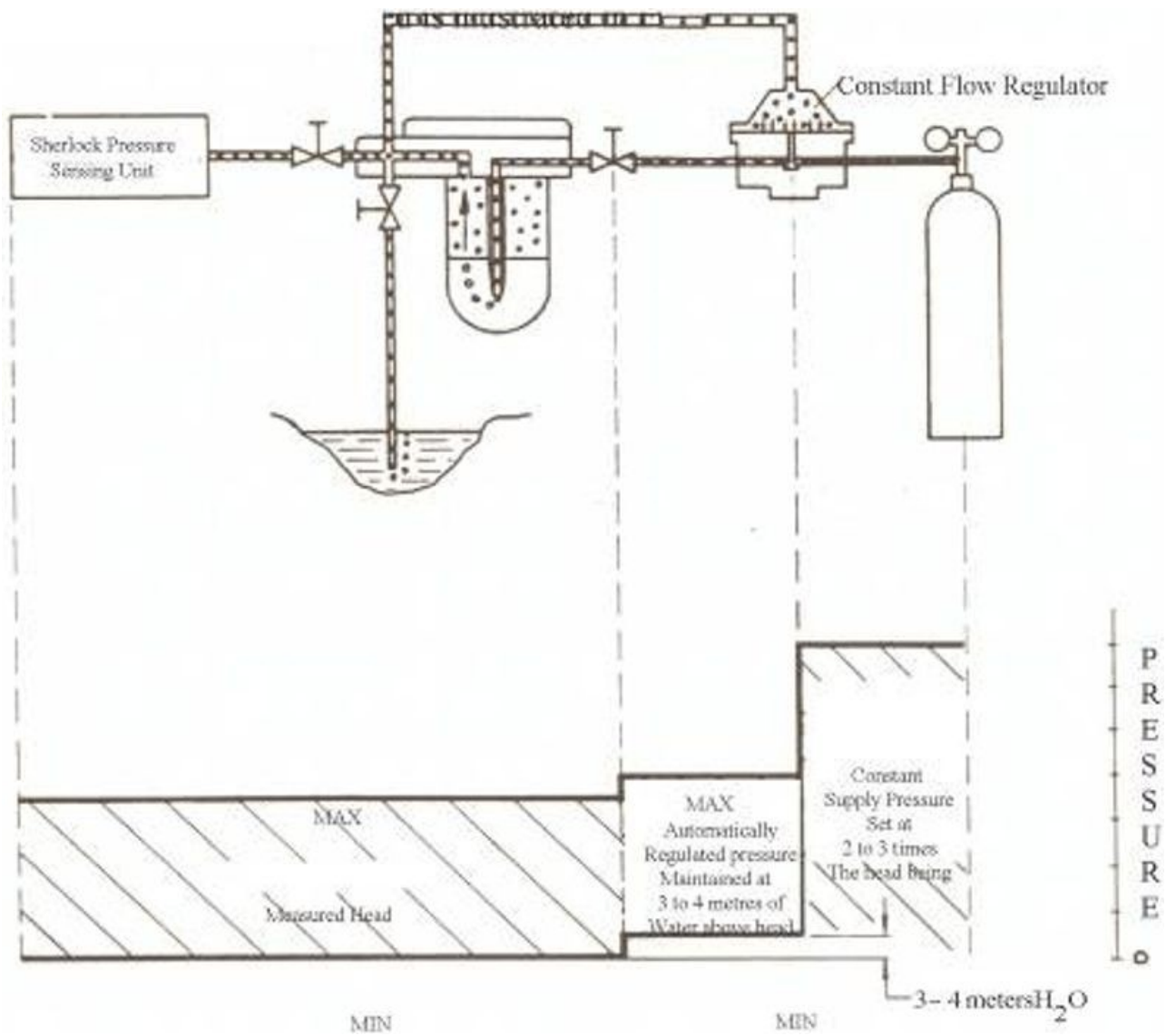
Figure 6 - Diagrammatic view of field gas purge, single line without purge facilities.
