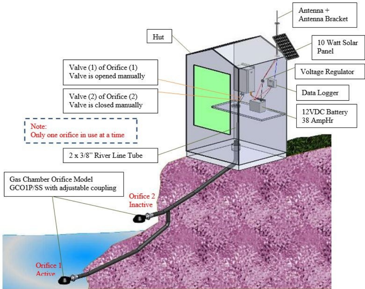
HS40 Compact-DO Typical Installation
